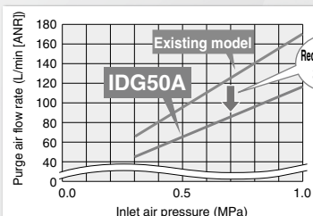
Purge air flow rate (rated conditions)
