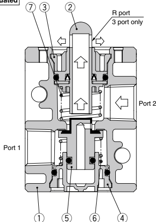
Non-actuated
