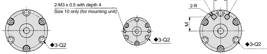
CRB2BW10-□S <Port position: Side ports>
