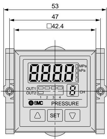
Front protective cover + Panel mount
