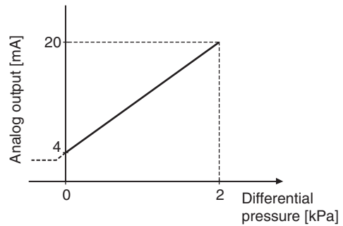
4 to 20 mADC
