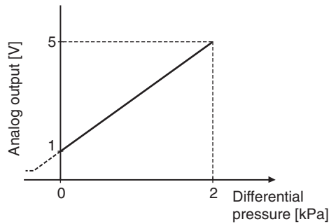
1 to 5 VDC
