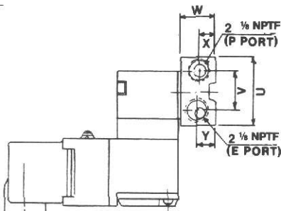
MANIFOLD DIMENSIONS
