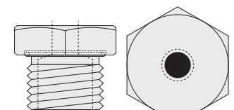
RB9/16-18-SAE x M6 x 1
