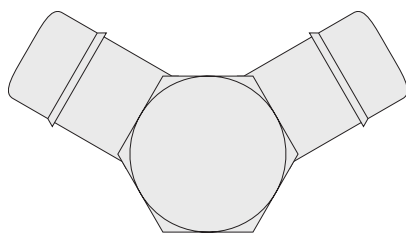
3/8FVT10-120°
