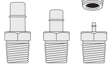
1/8B6 1/8B5 1/2 1/8B.045
