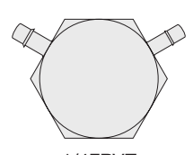
1/4FRVT 2-1-120°-RH
