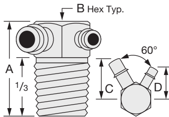
Top View: Right-hand Reducing VT's have the (smaller) Reducing Branch on the right.
