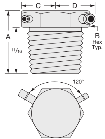
Top View: Right-hand Reducing 120° VT's have the smaller branch on the right.
