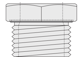
RB3/4BSPPx1/2BSPP
