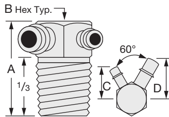
Top View: Left-hand Reducing VT's have the (smaller) Reducing Branch on the left.
