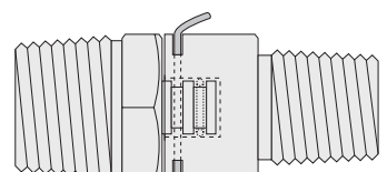
3/8RSWN-1/4-GT
