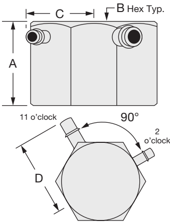
Top View: Right-hand Reducing 90° VT's have the hex flat branch on the right (2 o'clock) while the hex point branch is at 11 o'clock.
