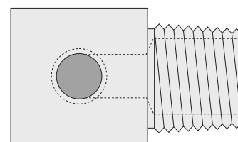
1/2BSPTx1/8-FL
