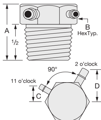
Top View: Left-hand Reducing 90° VT's have the hex point branch at 2 o'clock while the hex flat branch is on the left, at 11 o'clock.
