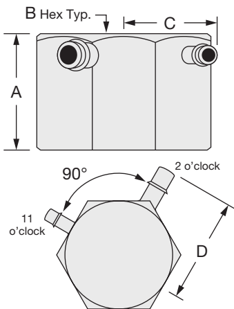
Top View: Left-hand Reducing 90° VT's have the hex flat branch on the left (11 o'clock) while the hex point branch is at 2 o'clock.
