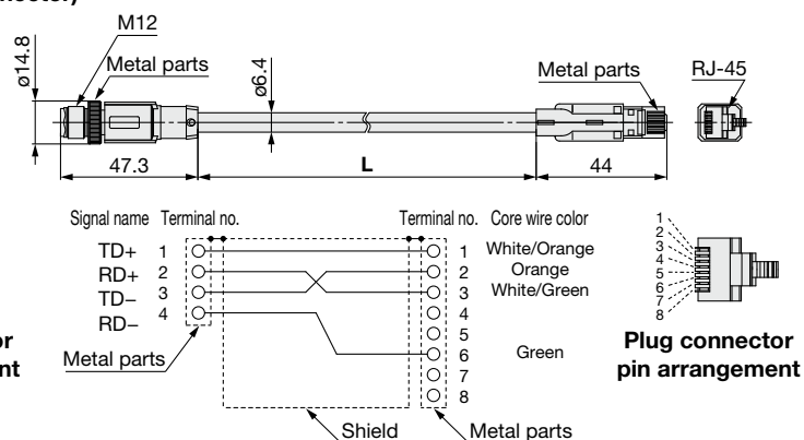
Connections (Straight cable)
