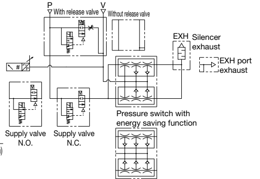
Circuit diagram
