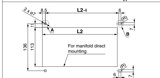
Panel cutout dimensions: Lead wire type
