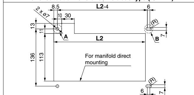
Panel cutout dimensions: Fieldbus type (IO-Link)
