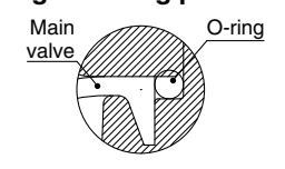
Fig. 2 O-ring position
