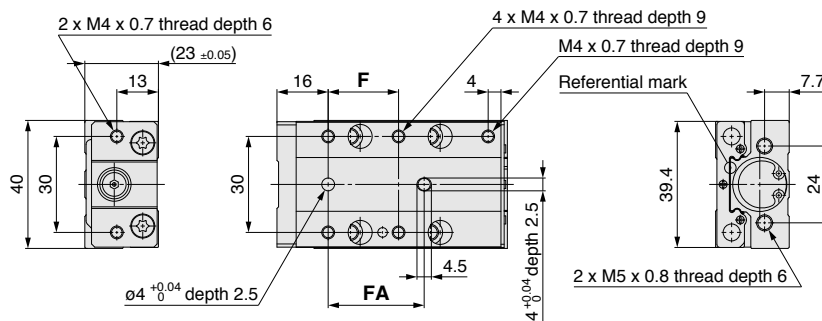
Dimensions taken from datum faces
