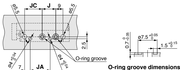
O-ring groove dimensions
