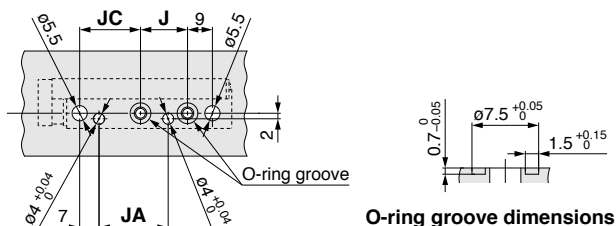
O-ring groove dimensions
