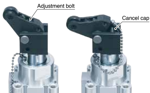
C Lever (Adjustable Absorber Type) with Cancel Cap
