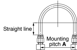
Fig. 1 Recommended piping
