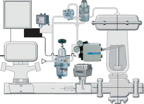
Instrumentation Typical pneumatic control system on a diaphragm valve using SMC pneumatic products.
