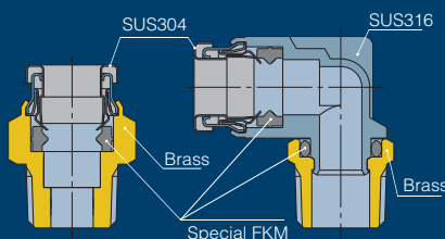
KQB2 Series The brass parts on the metal one-touch fitting are electroless nickel plated
