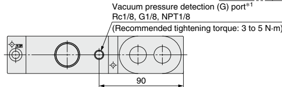
With vacuum pressure detection port
