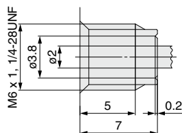
Details of thread
