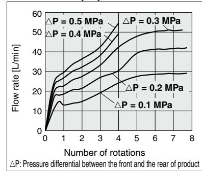
PF3W740S(-L)/540S
