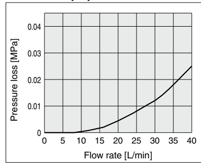
PF3W740(-L)/540
