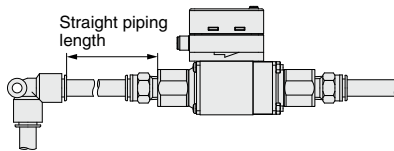
PF3W704(-L)/504 Pressure: 0.3 MPa Piping diameter: \phi 12
