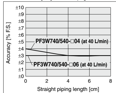
PF3W740(-L)/540 Pressure: 0.3 MPa Piping diameter: \phi 16
