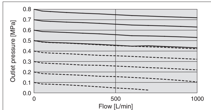
AW30-D + PF3A701H/PF3A801H-L
