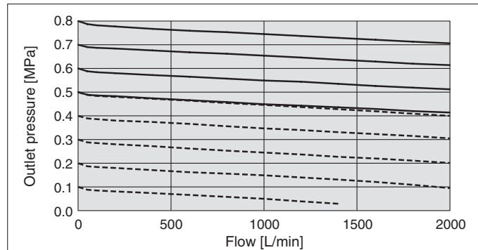
AW40-D + PF3A702H/PF3A802H-L
