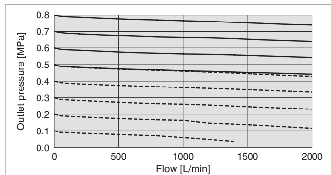
AW40-D + PF3A702H/PF3A802H-L
