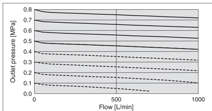
AW30-D + PF3A701H/PF3A801H-L
