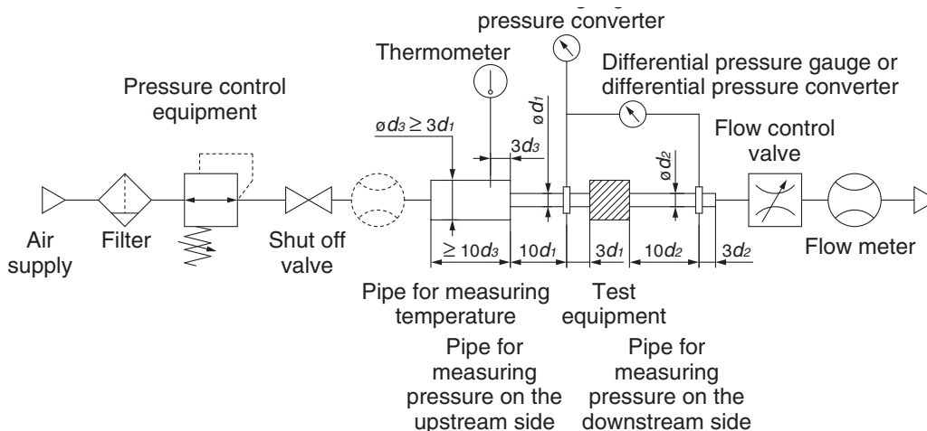
Fig. (1) Test circuit based on ISO 6358:1989, JIS B 8390:2000
