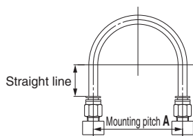
Fig. 1 Recommended piping
