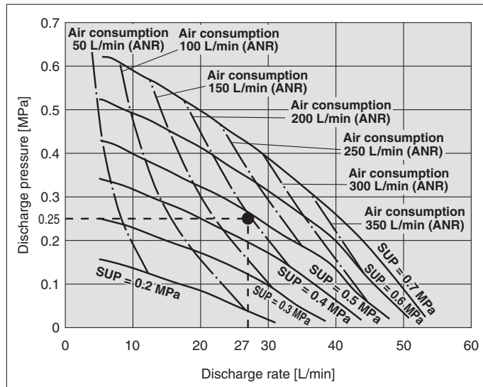
PA5010-□04 Flow Rate Characteristics
