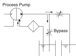
Circuit example (2)
