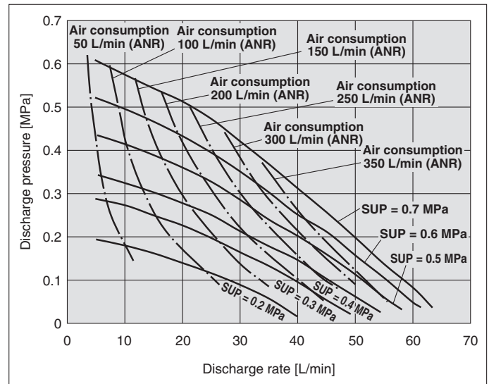
PA5010-□06 Flow Rate Characteristics
