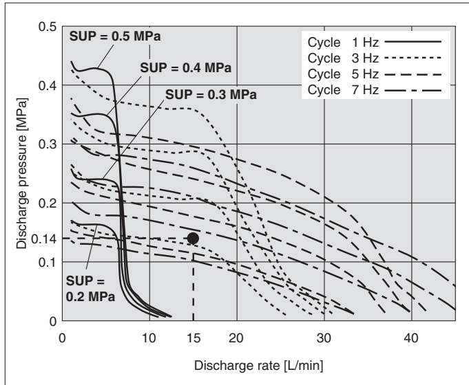
PA5 0 2 13-□04 Flow Rate Characteristics
