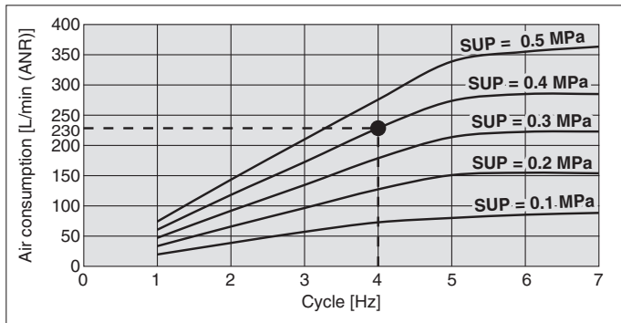
PA5 0 2 13 Air Consumption
