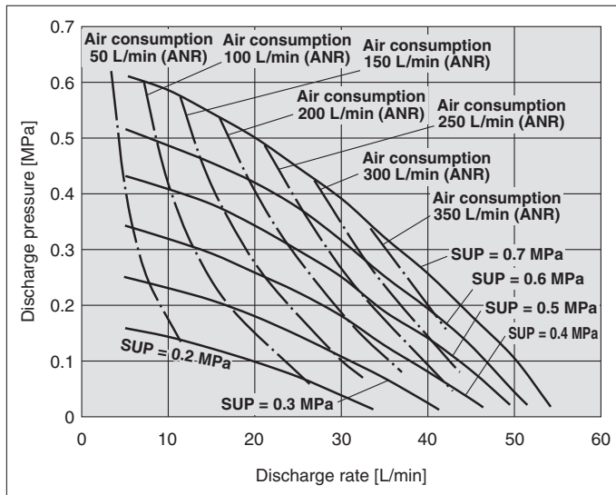
PA5010-13□04 Flow Rate Characteristics
