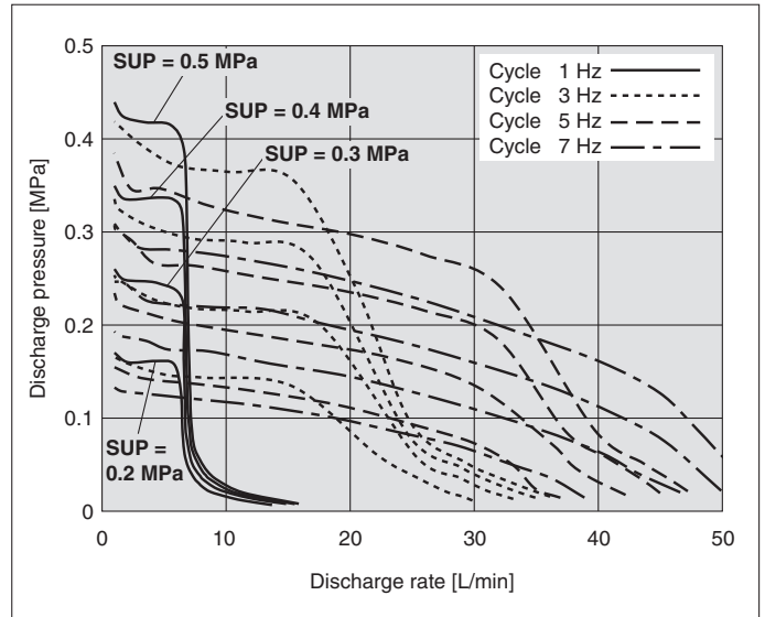
PA5 0 2 13-□06 Flow Rate Characteristics
