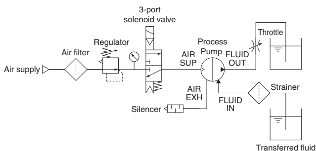
Circuit example (1)
