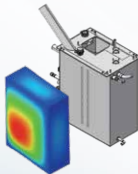
Tank assessments (withstand pressure testing and deformation simulations)
