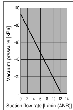
Flow Rate Characteristics (0.45 MPa)
