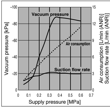
Exhaust Characteristics
