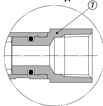
Screw-in type
