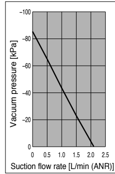
Flow Rate Characteristics (0.35 MPa)
