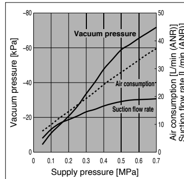
Exhaust Characteristics
