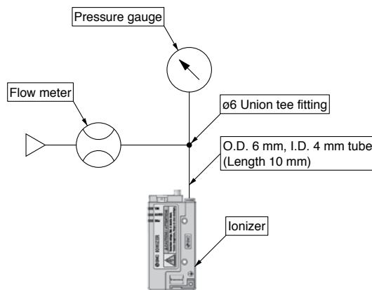
Fig. 1: Flow rate characteristics measuring circuit
