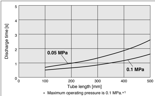
③ Female threads for piping IZN10E-11 With Stainless steel 316 One-touch fitting* 2 + Anti-static tubing
