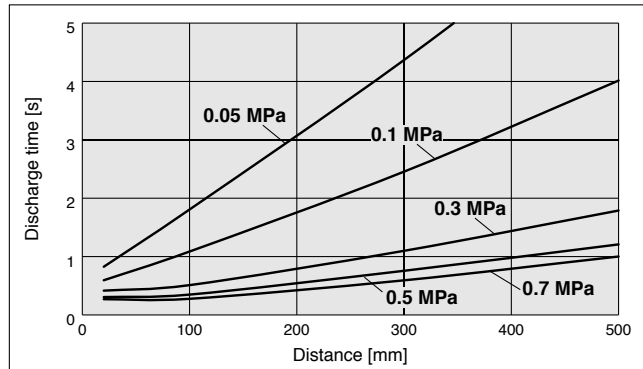
② High flow rate nozzle IZN10E-02-X367
