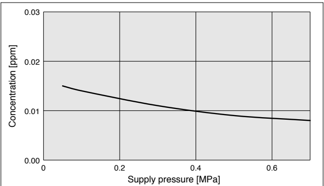
② High flow rate nozzle IZN10E-02
