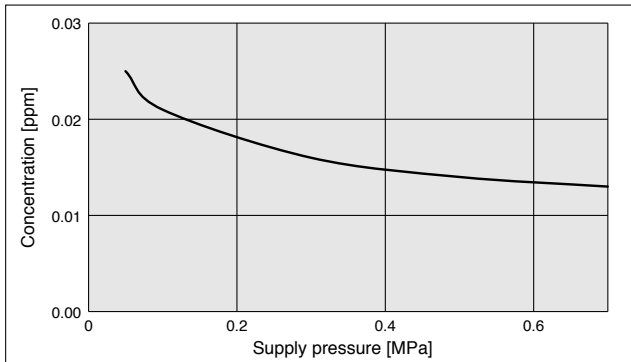
① Energy saving static neutralization nozzle IZN10E-01
