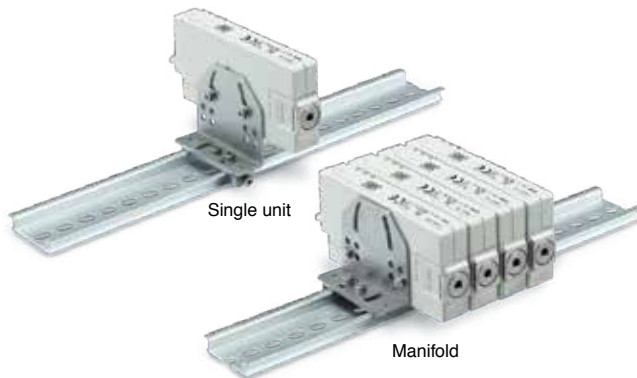
DIN rail mounting bracket
