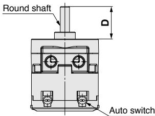
Single shaft/CDRBT□
