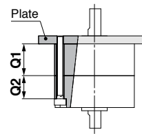
Body mounting 2 (Body through-hole)
