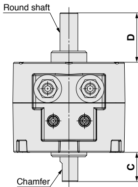
Double shaft/CRBJ□
