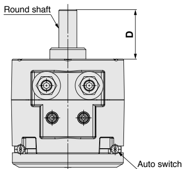
Single shaft/CDRBT□
