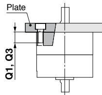
Body mounting 1 (Body tapped)
