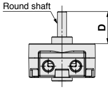
Single shaft/CRBT□
