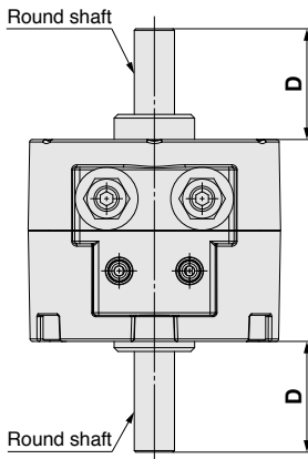
Double shaft/CRBK□
