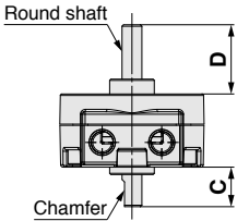
Double shaft/CRBJ□
