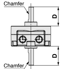
Double shaft/CRBY□
