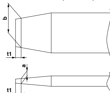
Screwdriver tip end shape
