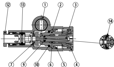
Section AA Meter-out
