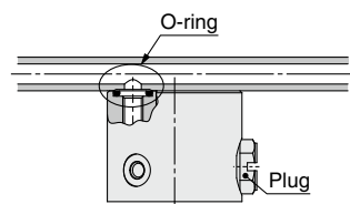
Requires no piping (Body ported)
