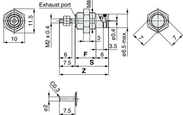
Without rod end thread CJPS4-□-B
