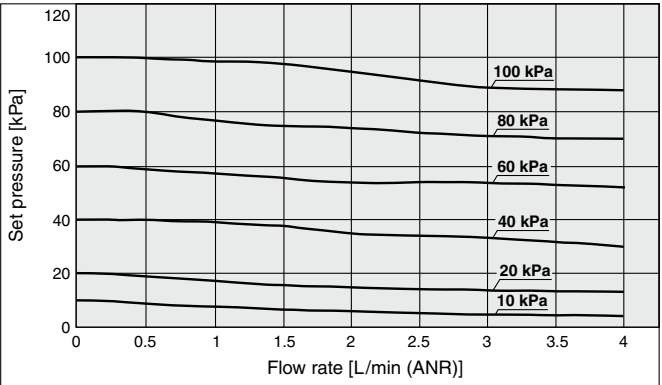
Flow Rate Characteristics
