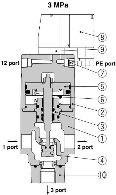
3-port valve
