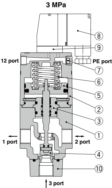
3-port valve (Dual pressure type)
