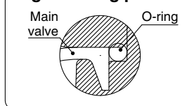
Fig. 2 O-ring position
