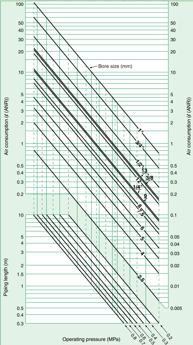
Graph (21) Air Consumption of Tube or Steel Pipe (For one cycle)
