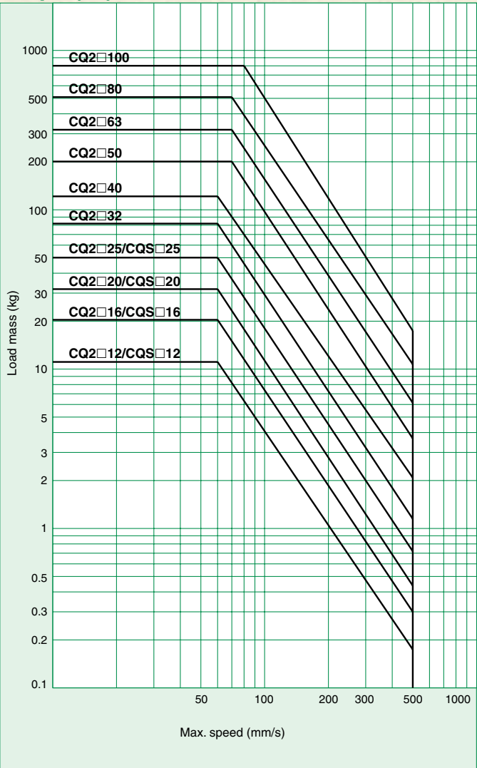
Graph (10) Series CQ2/CQS
