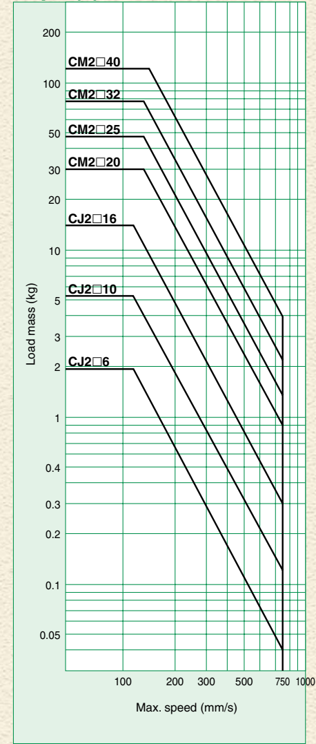
Graph (7) Series CJ2/CM2
