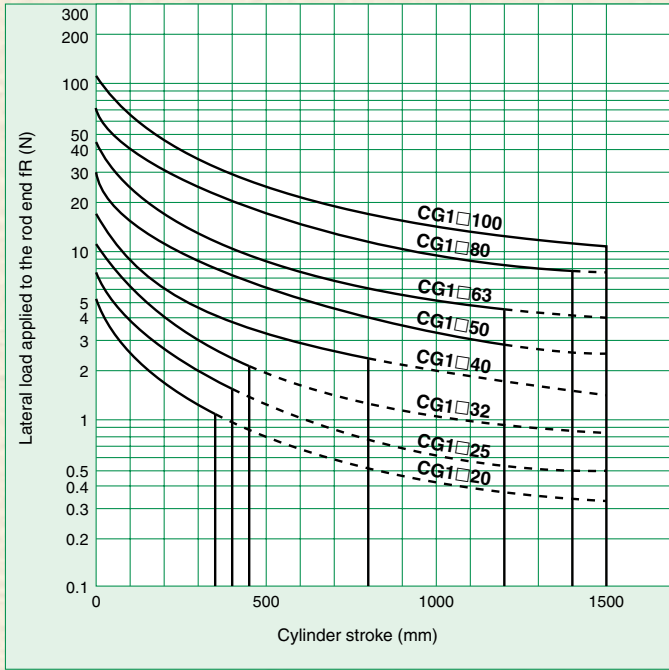
Graph (13) Series CG1: ø20, ø25, ø32, ø40, ø50, ø63, ø80, ø100
