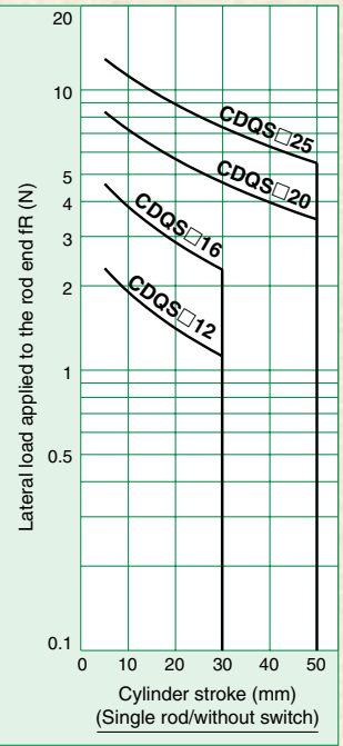
Graph (17) Series CDQS: ø12, ø16, ø20, ø25
