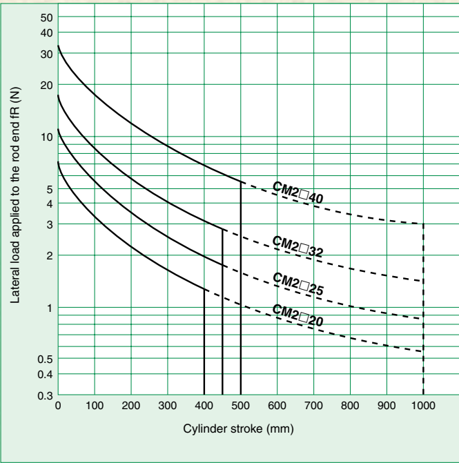
Graph (12) Series CM2: ø20, ø25, ø32, ø40
