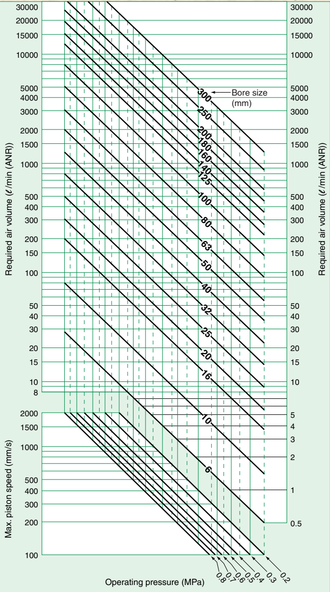
Graph (22) Required Air Volume of Cylinder and Piping
