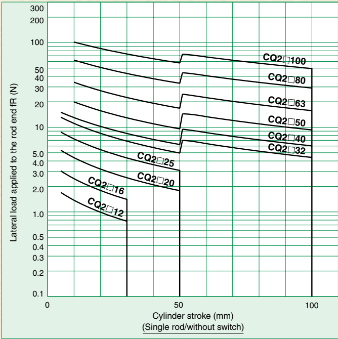
Graph (18) Series CQ2: ø12, ø16, ø20, ø25, ø32, ø40, ø50, ø63, ø80, ø100
