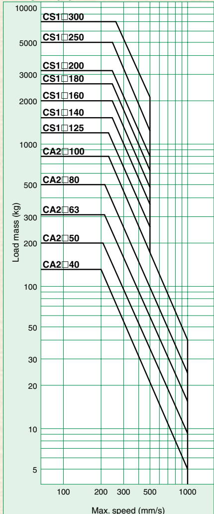
Graph (5) Series CA2/CS1
