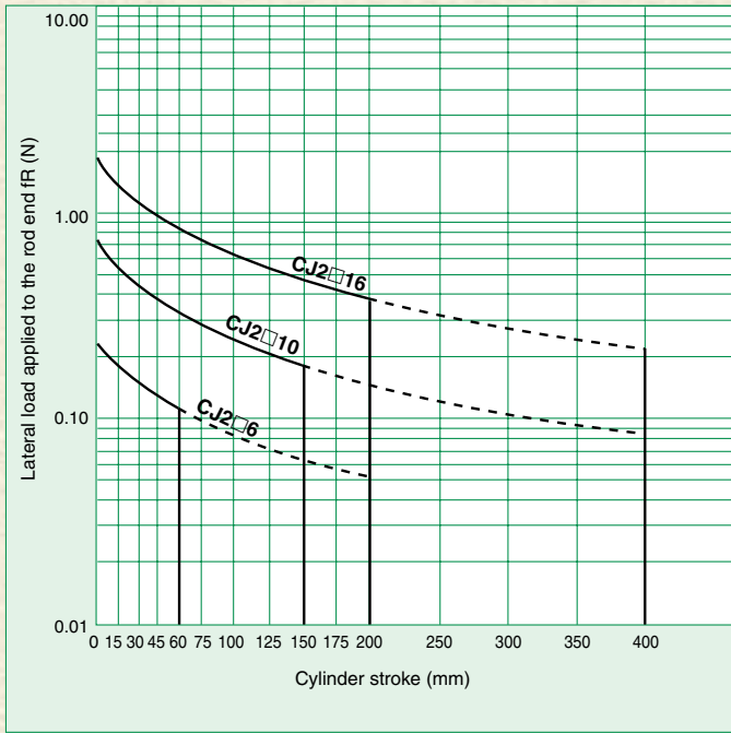
Graph (11) Series CJ2: ø6, ø10, ø16
