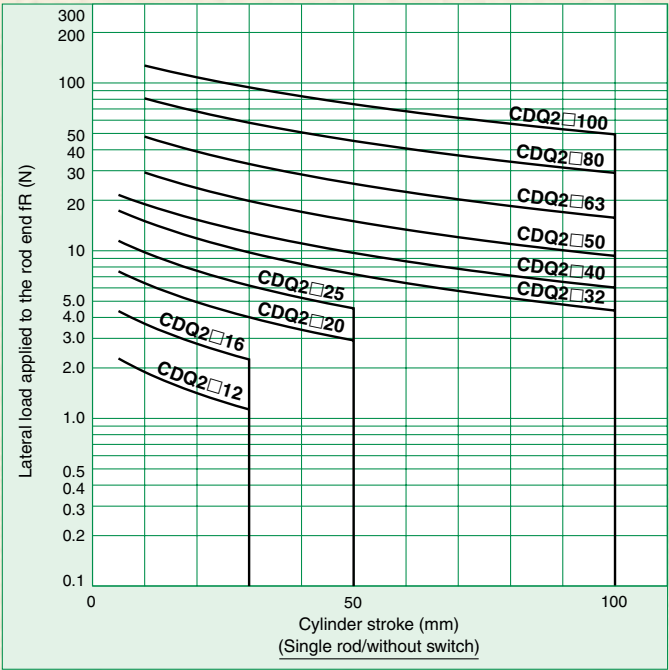
Graph (19) Series CDQ2: ø12, ø16, ø20, ø25, ø32, ø40, ø50, ø63, ø80, ø100
