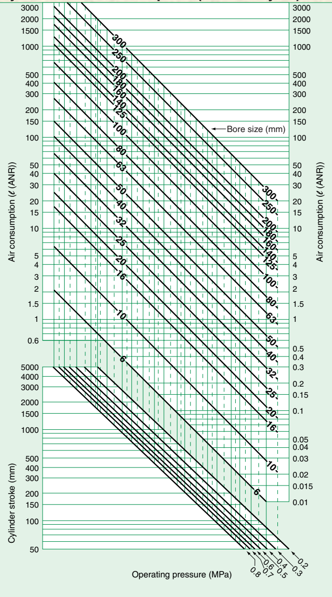
Graph (20) Cylinder's Air Consumption (For one cycle)
