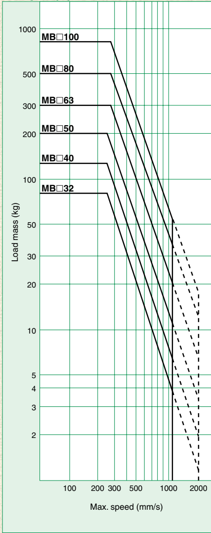
Graph (6) Series MB
