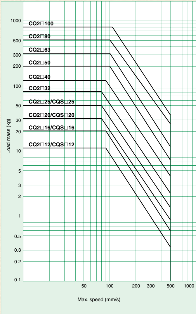
Graph (9) Series CQ2/CQS
