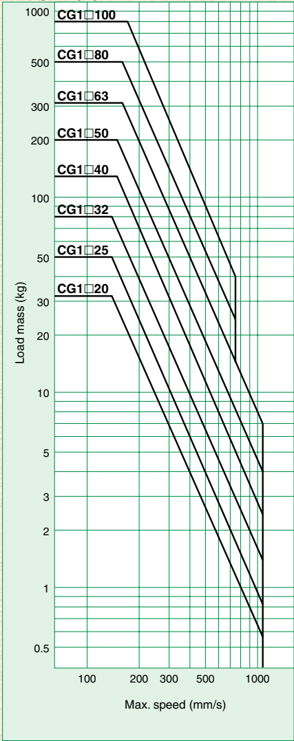
Graph (8) Series CG1
