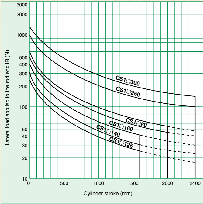
Graph (15) Series CS1: ø125, ø140, ø160, ø180, ø200, ø250, ø300
