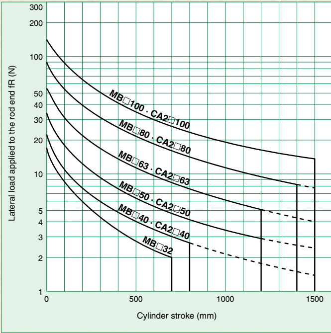
Graph (14) Series MB: ø32, ø40, ø50, ø63, ø80, ø100 Series CA2: ø40, ø50, ø63, ø80, ø100
