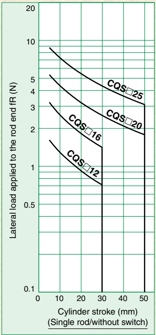
Graph (16) Series CQS: ø12, ø16, ø20, ø25
