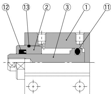
Without magnet
