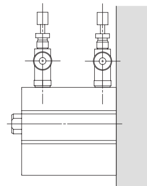
Mounting condition 4
