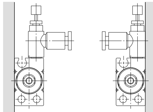
Mounting condition 1
