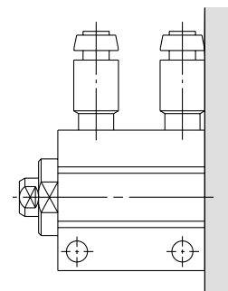
Mounting condition 4
