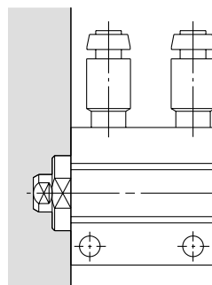
Mounting condition 3
