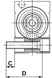
Lateral mounting
