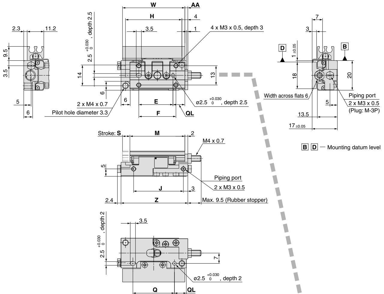
Without magnet and switch rail
