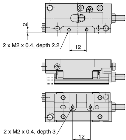
Without magnet and switch rail
