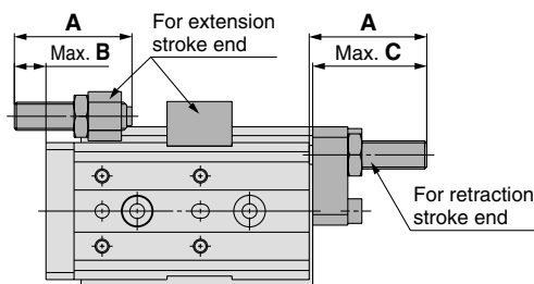
Rubber Stopper (AS, AT, A) (mm)
