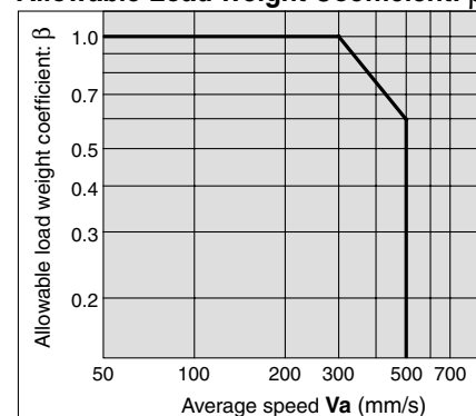
Graph (1) Allowable Load Weight Coefficient: \beta
