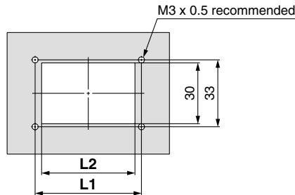
Panel fitting dimensions/Mounting hole dimensions
