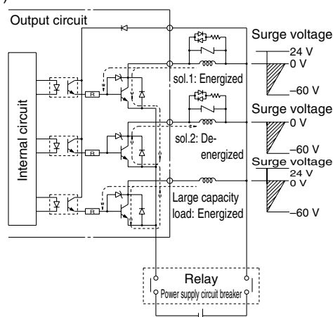
Figure 1. Surge intrusion circuit example (24 VDC)
