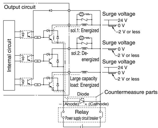
Figure 2. Surge intrusion circuit example (24 VDC)
