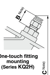
One-touch fitting mounting (Series KQ2H)
