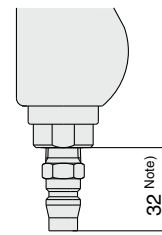
S coupler plug mounting (KK130P-02MS)
