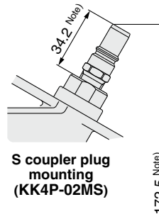
S coupler plug mounting (KK4P-02MS)
