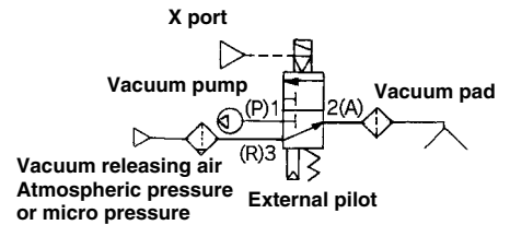
External pilot
