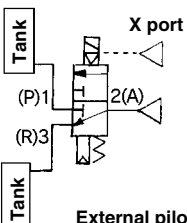
External pilot
