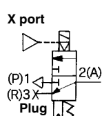
External pilot
