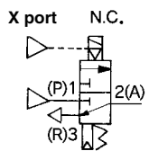
External pilot
