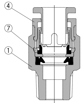
Male connector
