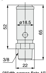
Safety valve VBAT-R, VBAT-S*
