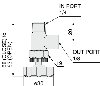
Drain valve VBAT-V1*
