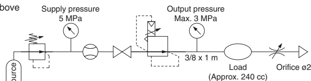
Fig. 1. Piping schematic
