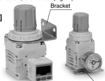
Bottom bracket
