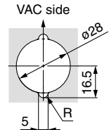
Panel cut
