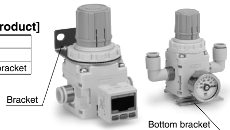
Bottom bracket
