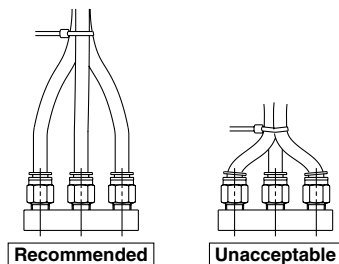
Fig. 2 Binding tubes with bands
