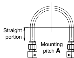
Fig. 1 Recommended piping configuration
