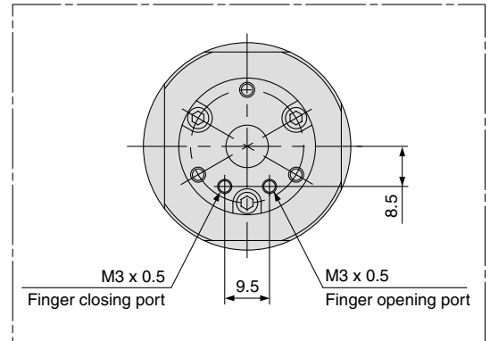
MDHR3-10E Port Location
