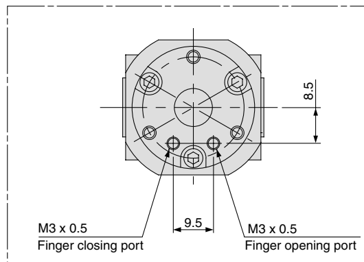
MDHR2-10E Port Location
