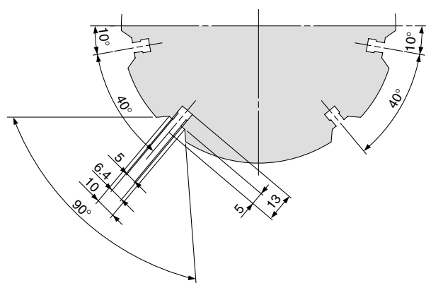
MHS3-100D
