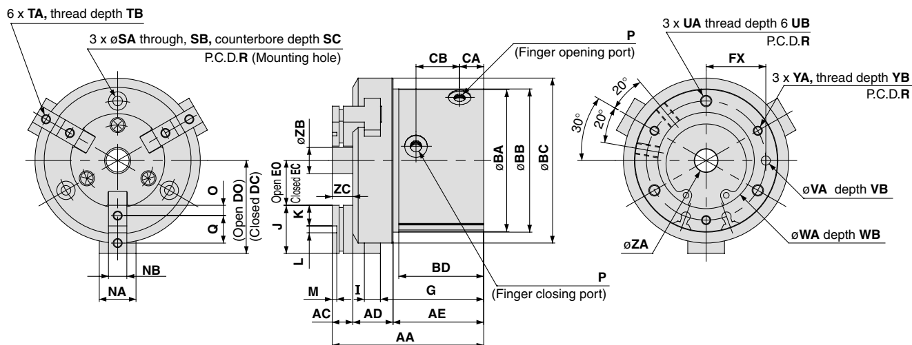
MHSH3-32D
