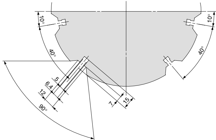
MHS3-125D
