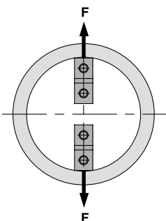
Internal grip
