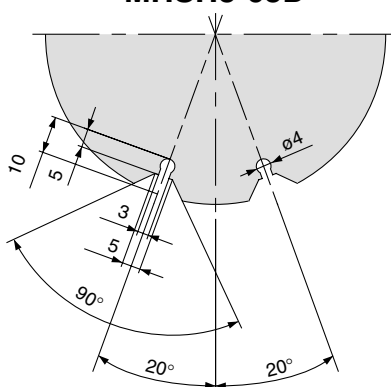
MHSH3-63D
