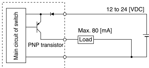
Fig. (4) Connection example of PNP output
