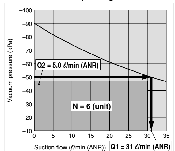
Chart 2. Example of Selection from Minimum Operating Flow
