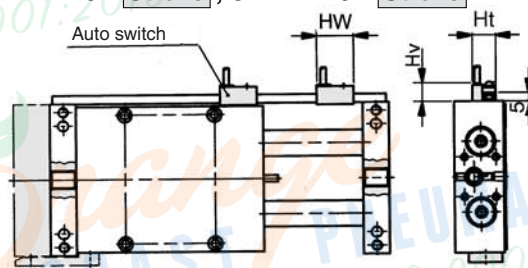
Plate mounting style with auto switch
