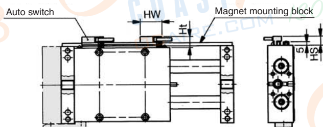
Housing mounting style with auto switch CDBXWL32-Stroke , CDBXWL32-Stroke R
